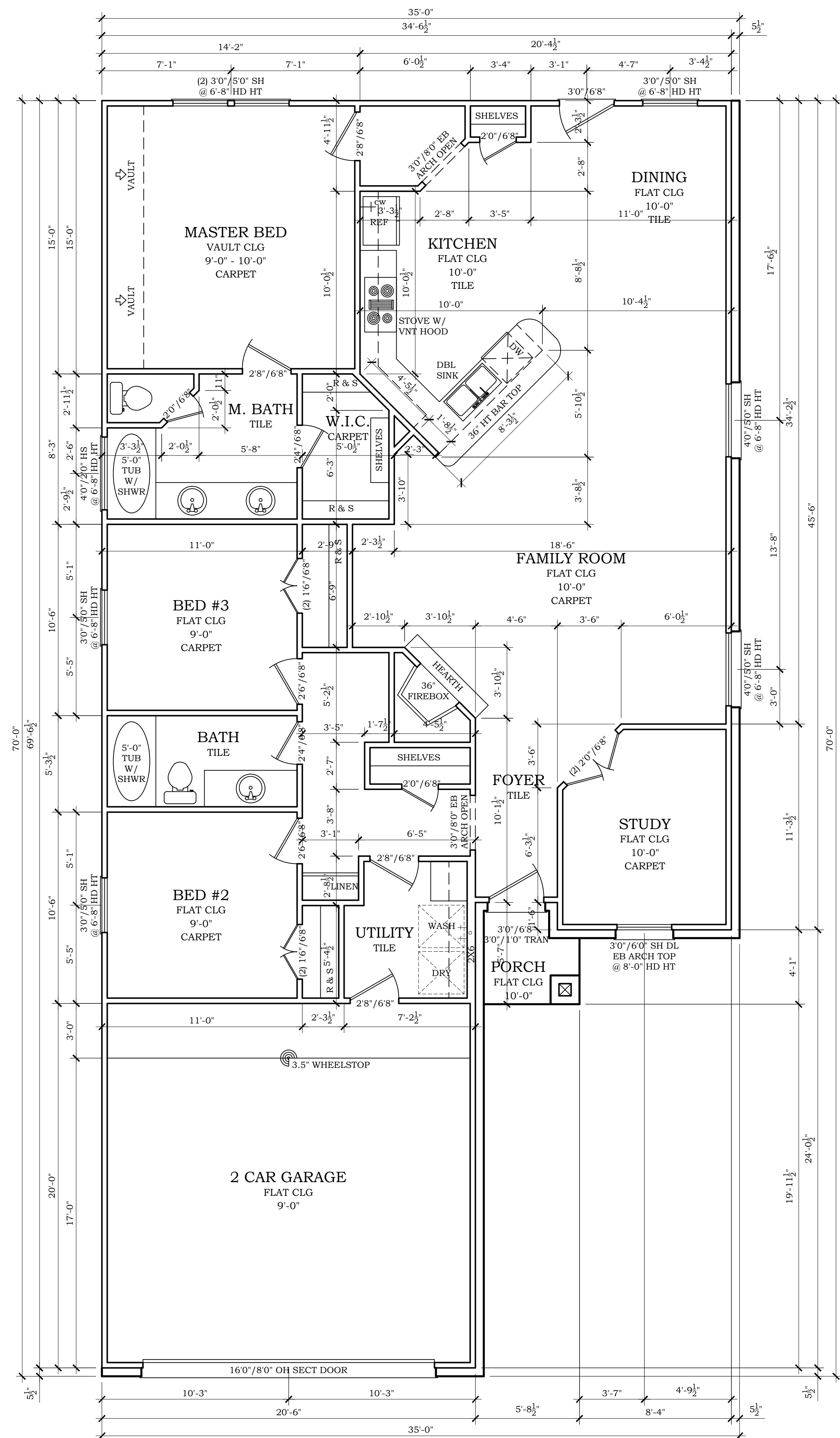
1 FLOOR PLAN A2 SCALE: 1/4" = 1'
