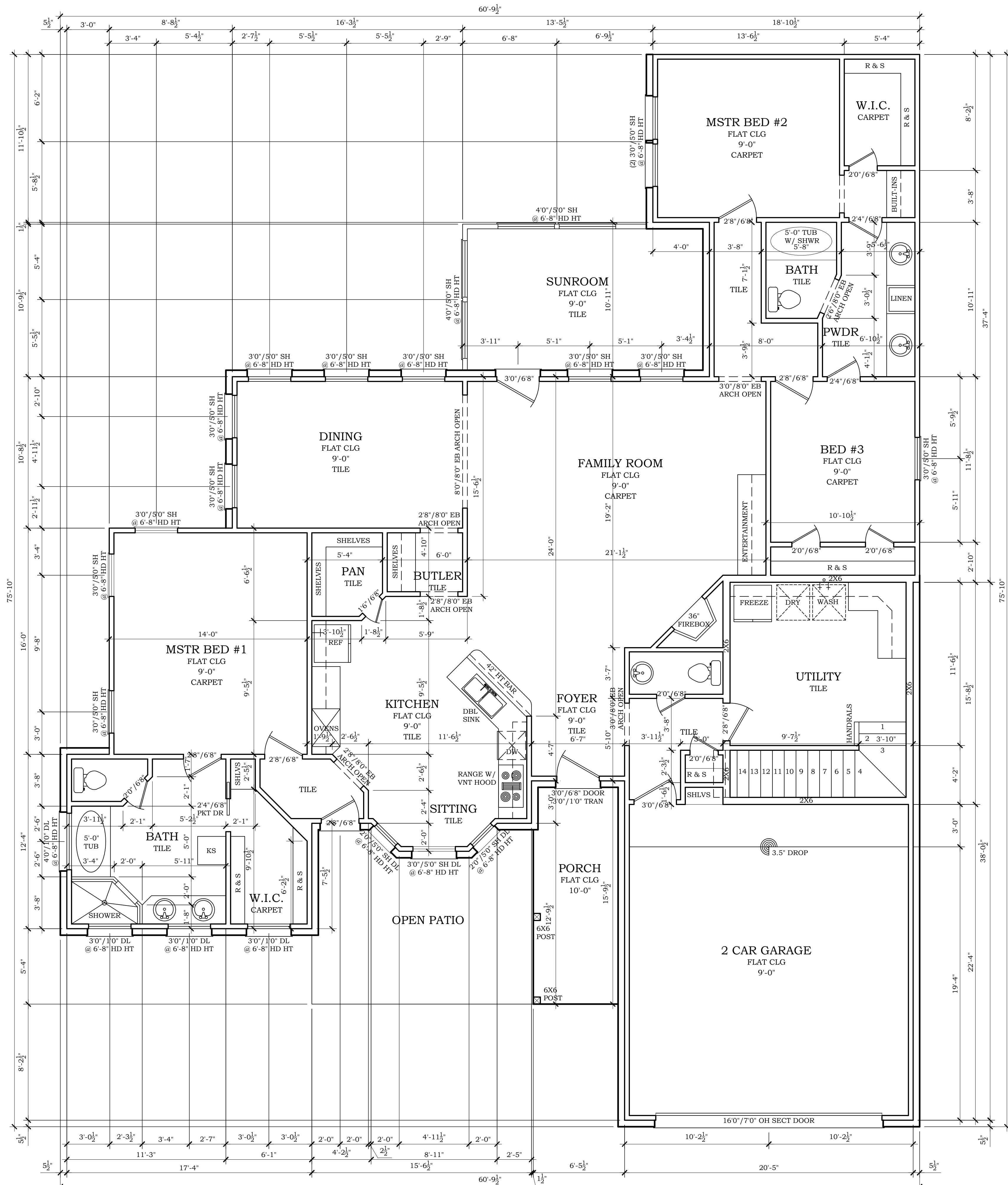
1 FLOOR PLAN A2 SCALE: 1/4" = 1'
